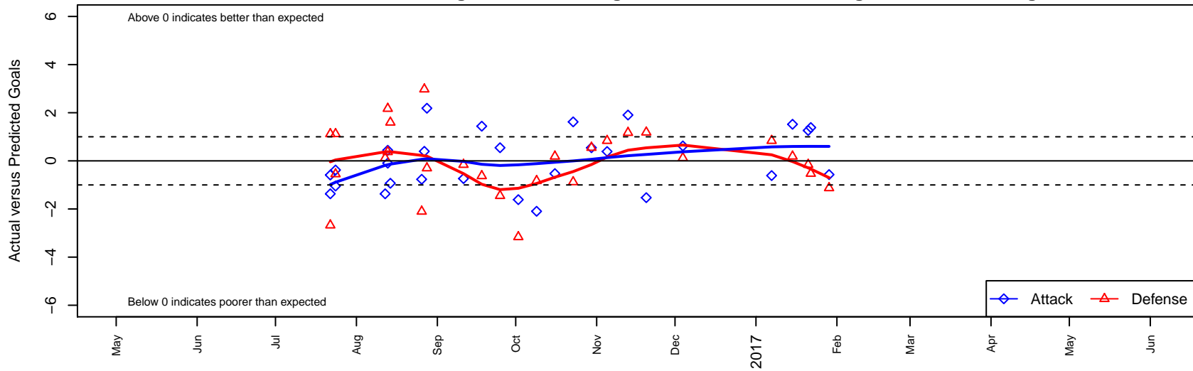
Crossfire Select Elder B00 Dots are actual minus expected GF (blue circles) and GA (red triangles). Blue line is smoothed change in attack strength. Red is smoothed change in defense strength.
